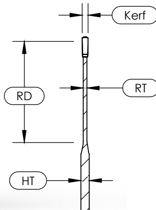
Glue-Line Rip
