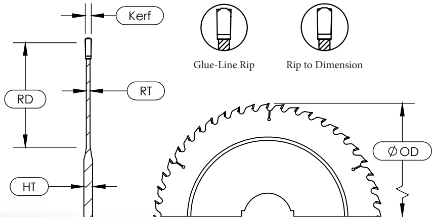
Typical HT(Hub Thickness) 3.00mm
