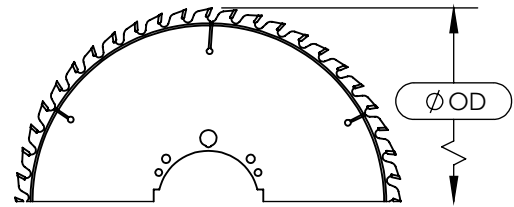
Typical HT (Hub Thickness) 3.00mm
